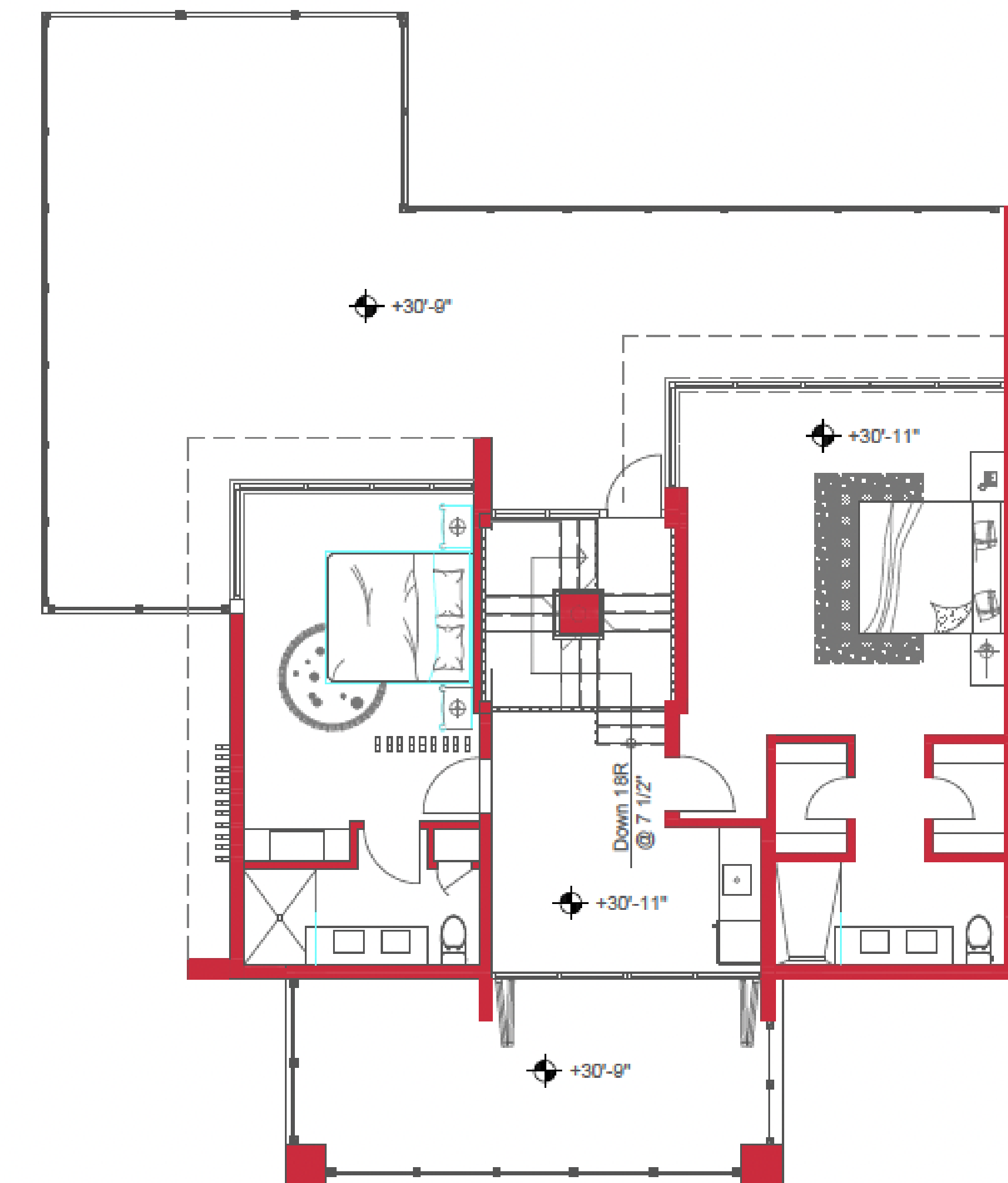
THIRD FLOOR
