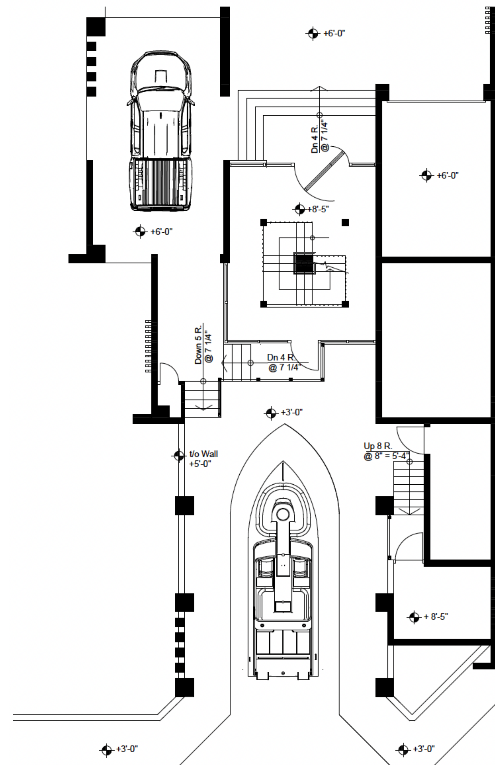
FIRST FLOOR
