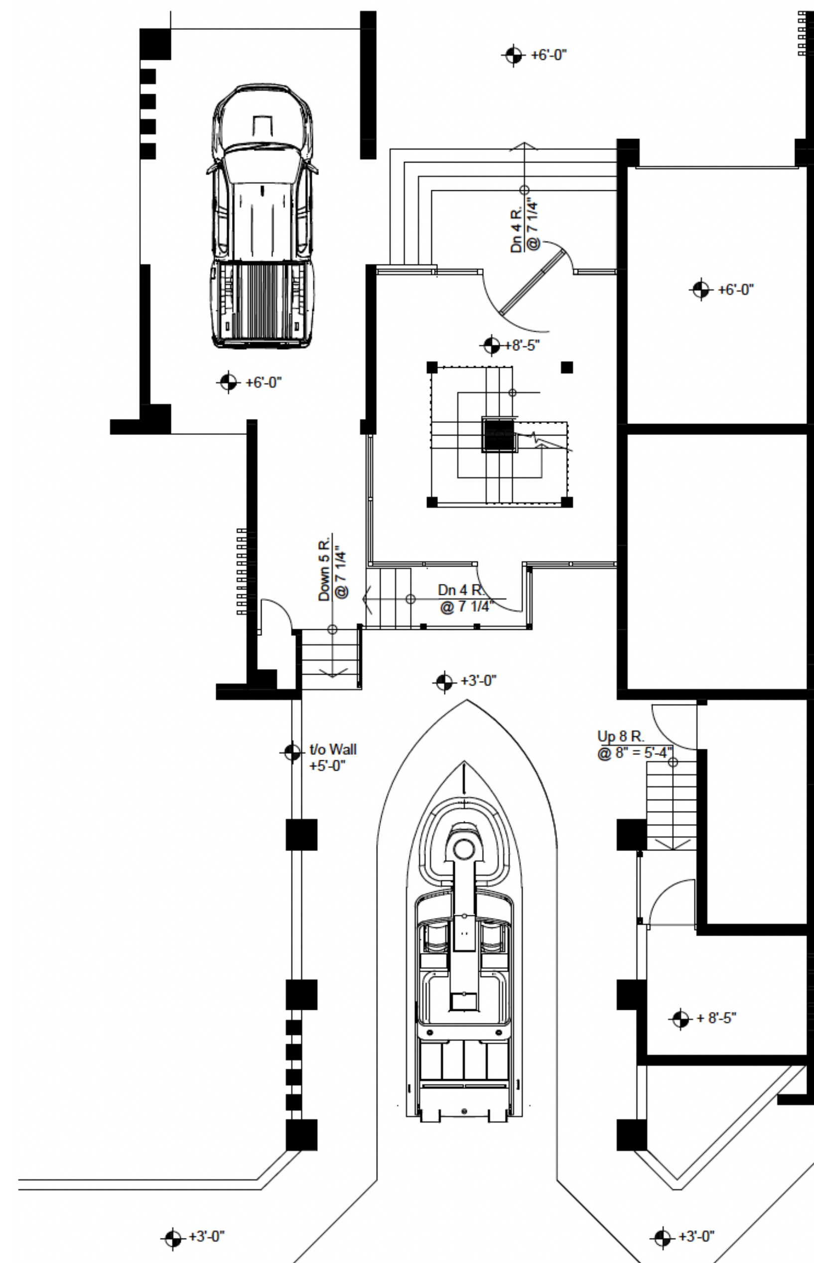
FIRST FLOOR
